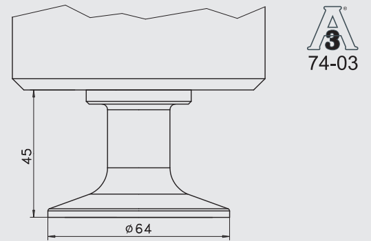
Dimensioned Drawing nozzle ITM-3 / TC2
